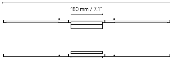
Double 960 mm / 37.8"
